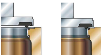
Principle of secondary force connection
