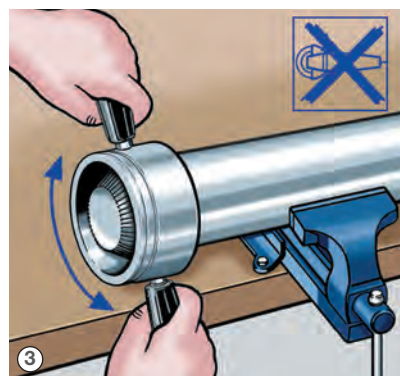
③ De-burr pipe internally and externally.
