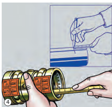
④ Mark the insertion depth. \varnothing 64.0 \text{ mm} = 43 \text{ mm} \varnothing 76.1 \text{ mm} = 50 \text{ mm} \varnothing 88.9 \text{ mm} = 50 \text{ mm} \varnothing 108.0 \text{ mm} = 60 \text{ mm}
