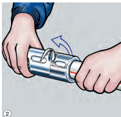
2 Dismantle the pipe end with the pipe dismantler.
