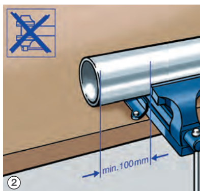
② Use the vice with caution! The end of the pipe must be perfectly round.
