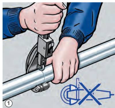
① Cut the pipe to length at a right angle.
