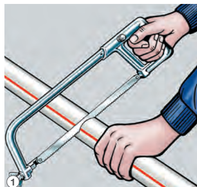
1 Stripped Prestabo-pipe cut the pipe to length at as near to a right angle as possible with a fine toothed saw.
