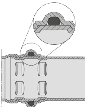
The sealing element is well protected at all times.
