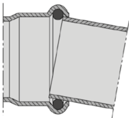
If the pipe guide is not cylindrical, the sealing element can be damaged.
