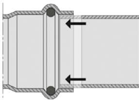
The Viega Profipress cylindrical pipe guide effectively prevents damage during installation.
