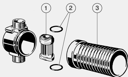
Insert - for concealed pipe interrupter - fig. 1 Model 6161.82
